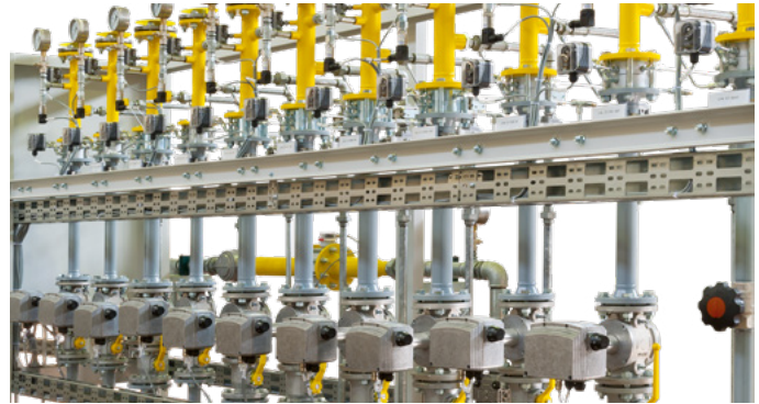
Mixing system in the glass industry
